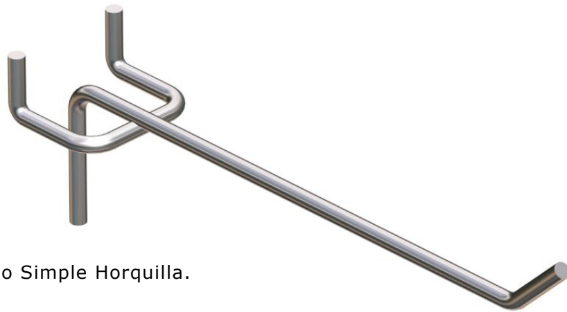
2. Ref.GSHOQ415 Gancho Simple Horquilla. Varilla 6ø x 400mm
